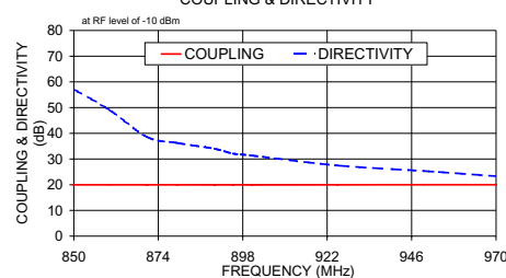
PDC20-970HP COUPLING & DIRECTIVITY
