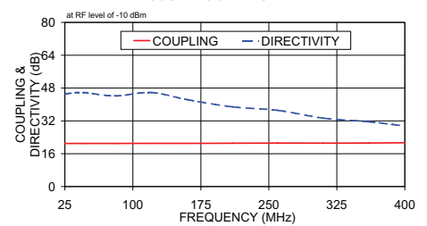
PDC-20-1 COUPLING & DIRECTIVITY
