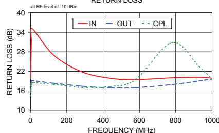
PDC-10-21+ RETURN LOSS
