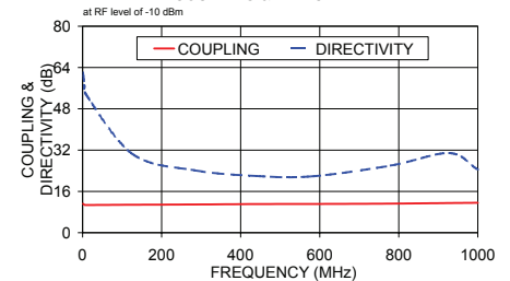
PDC-10-21+ COUPLING & DIRECTIVITY
