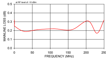
ZDC-20-3 MAINLINE LOSS
