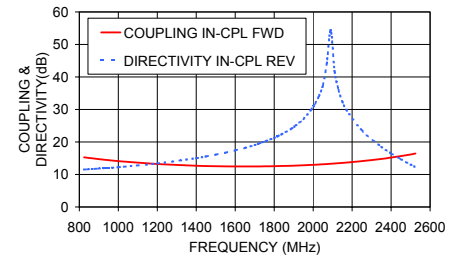
BDCN-15-25 COUPLING & DIRECTIVITY
