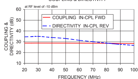
SYDC-30-12HP+ COUPLING & DIRECTIVITY
