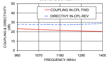
SYBD-20-142HP+ COUPLING & DIRECTIVITY
