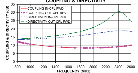
BDCN-10-25+ COUPLING & DIRECTIVITY
