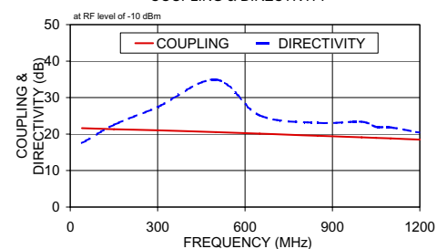
TCD-20-4-75+ COUPLING & DIRECTIVITY
