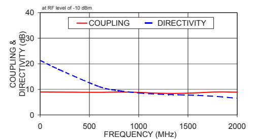
COUPLING & DIRECTIVITY
