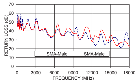
141-15SM+ RETURN LOSS
