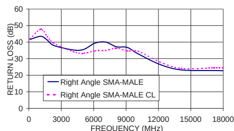
086-6SMRC+ RETURN LOSS
