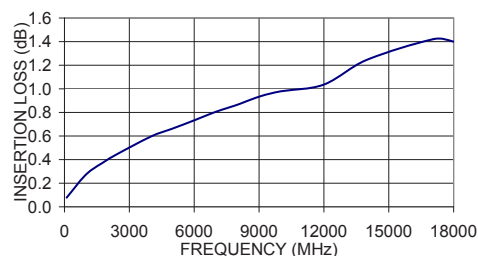
086-14SMR+ INSERTION LOSS
