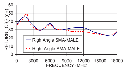
086-14SMR+ RETURN LOSS
