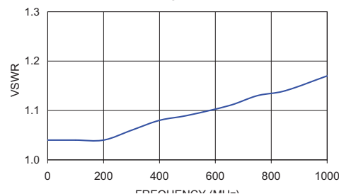
LAT-30+ VSWR
