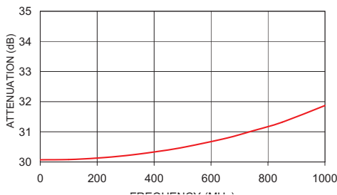
LAT-30+ ATTENUATION
