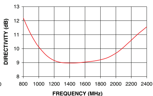
ZX60-2411BM+ DIRECTIVITY
