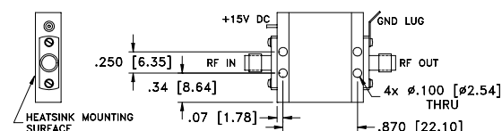
MOUNTING INFORMATION FOR MODELS WITHOUT HEATSINK
