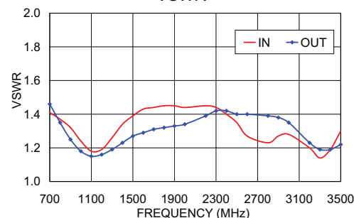
ZRL-3500+ VSWR
