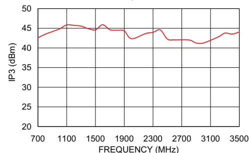
ZRL-3500+ IP3
