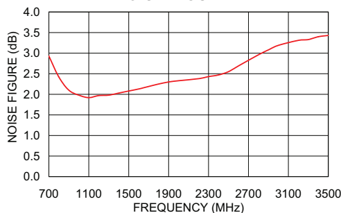
ZRL-3500+ NOISE FIGURE
