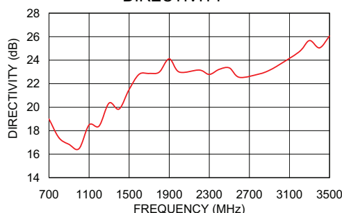
ZRL-3500+ DIRECTIVITY
