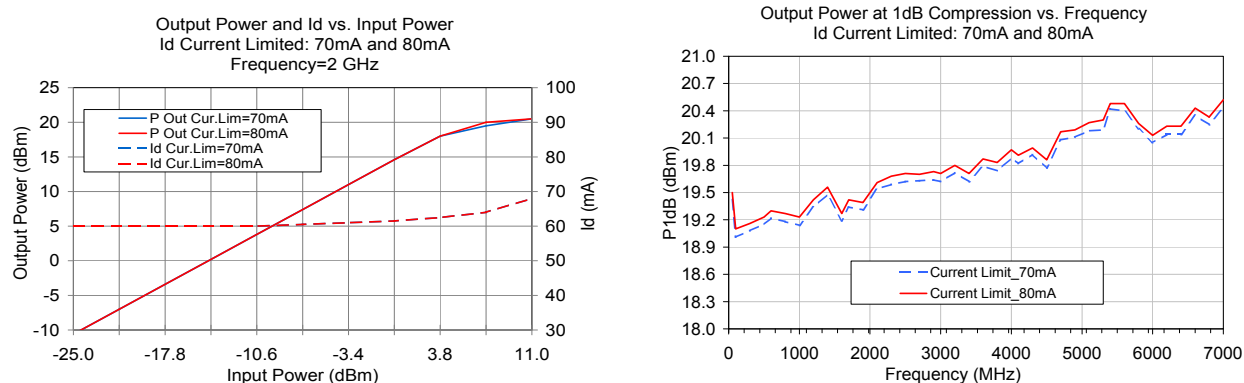
Fig 2. Output Power and I_d vs. Input Power and Frequency. Performance measured on Mini-Circuits Characterization test board TB-502+. See Characterization Test Circuit (Fig. 1) Measurements performed with current ( I_d ) limited as noted.
