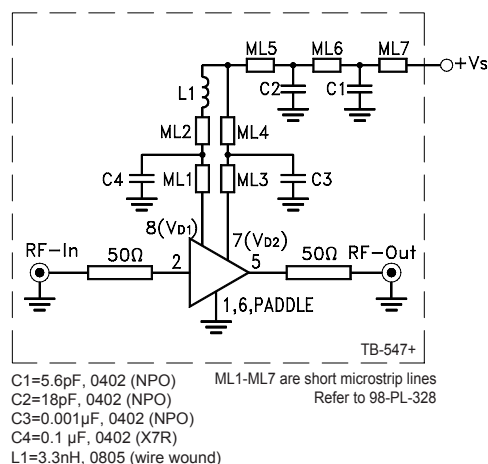
Fig 1. Block Diagram of Test Circuit used for characterization. (DUT soldered on Mini-Circuits Characterization Test Board TB-547+) Gain, Output power at 1dB compression (P1dB), Noise Figure, Output IP3 (OIP3) are measured using Agilent's N5242A PNA-X microwave network analyzer.
