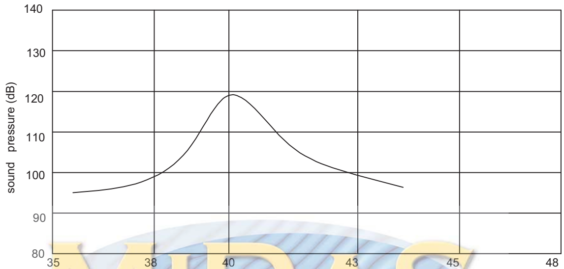
Frequency(kHz) SPL-Freq.Characteristics Frequency(kHz) Sensitivity-Freq.Characteristics
