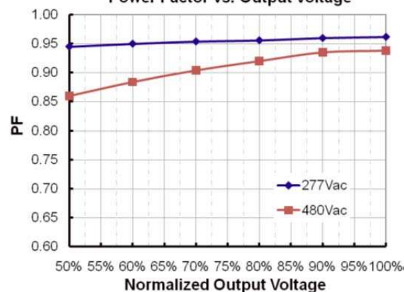
Power Factor vs. Output Voltage
