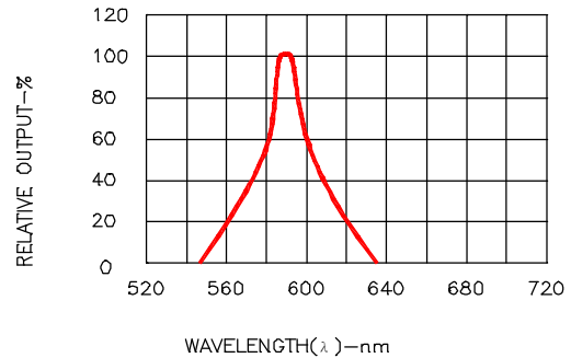
Fig.2 SPECTRAL RESPONSE
