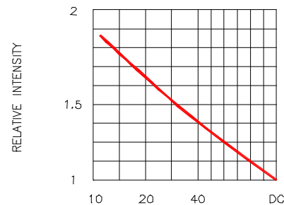
Fig.4 LUMINOUS INTENSITY VS. DUTY CYCLE (AVERAGE I_f = 10\text{mA} )
