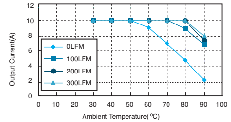
Figure 3. Typical Power De-rating for 12V IN
