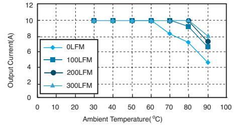
Figure 2. Typical Power De-rating for 12V IN
