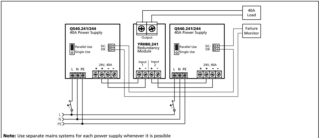
Fig. 18-2 Wiring diagram, 1+1 Redundancy, 40A output current
