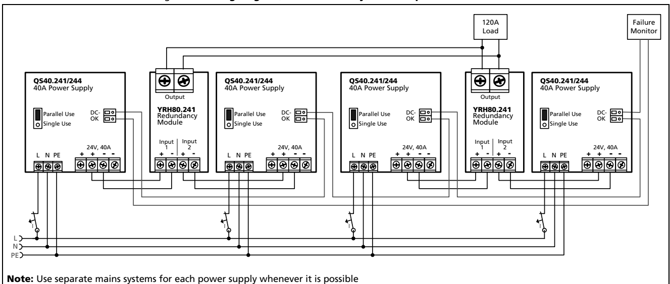
Fig. 18-3 Wiring diagram, n+1 Redundancy, 120A output current
