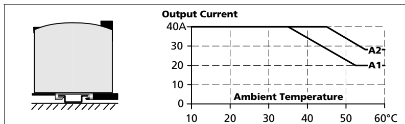
Fig. 19-6 Mounting Orientation C (Table-top mounting)
