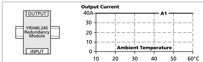
Fig. 19-4 Mounting Orientation A (Standard orientation)
