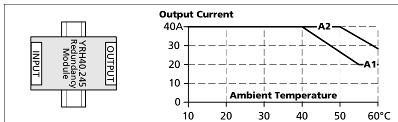
Fig. 19-7 Mounting Orientation D (Horizontal cw)
