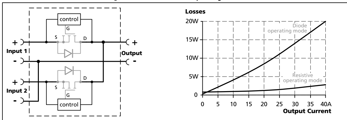
Fig. 19-1 Resistive vs. diode operating mode
