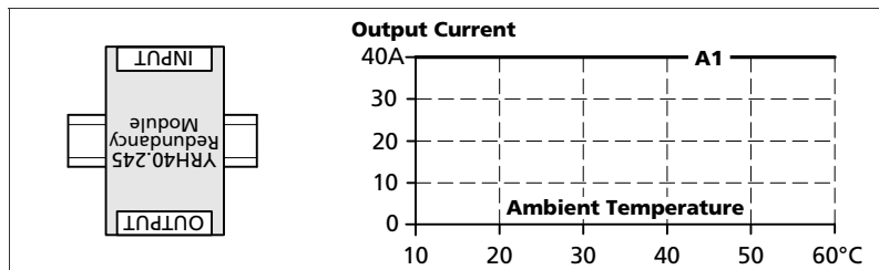
Fig. 19-5 Mounting Orientation B (Upside down)
