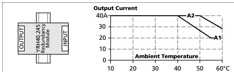
Fig. 19-8 Mounting Orientation E (Horizontal ccw)
