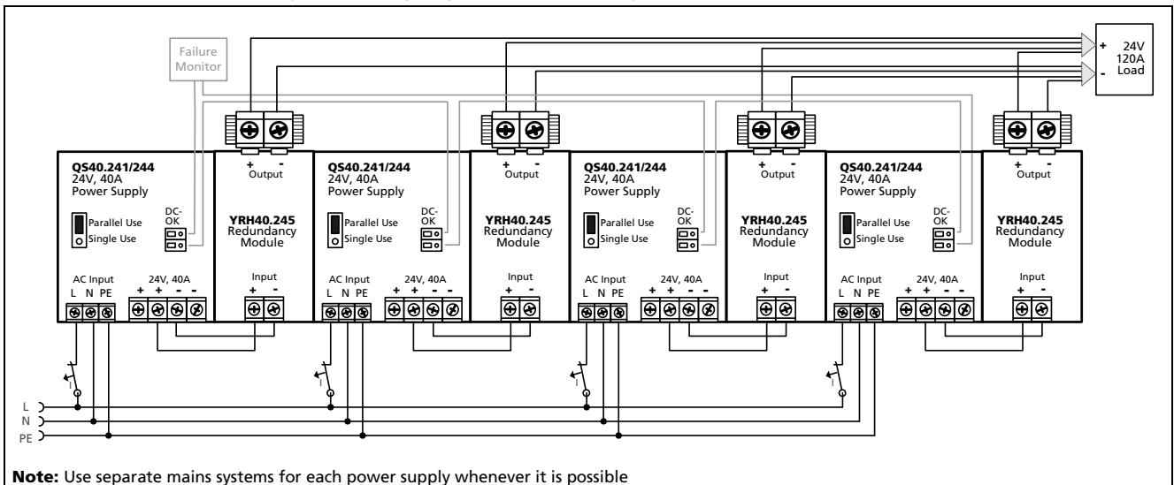
Fig. 19-3 Wiring diagram, n+1 Redundancy, 120A output current
