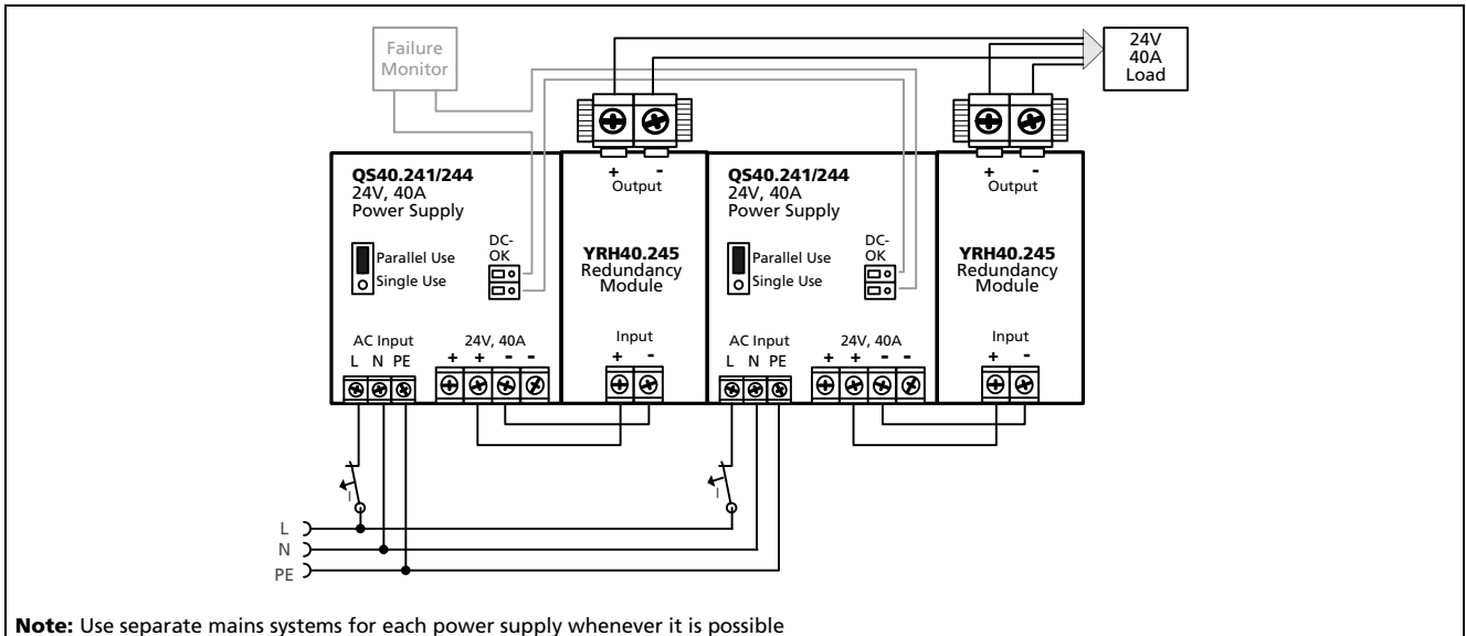
Fig. 19-2 Wiring diagram, 1+1 Redundancy, 40A output current
