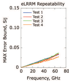
Highly-repeatable LRRM calibration algorithm available from WinCal XE
