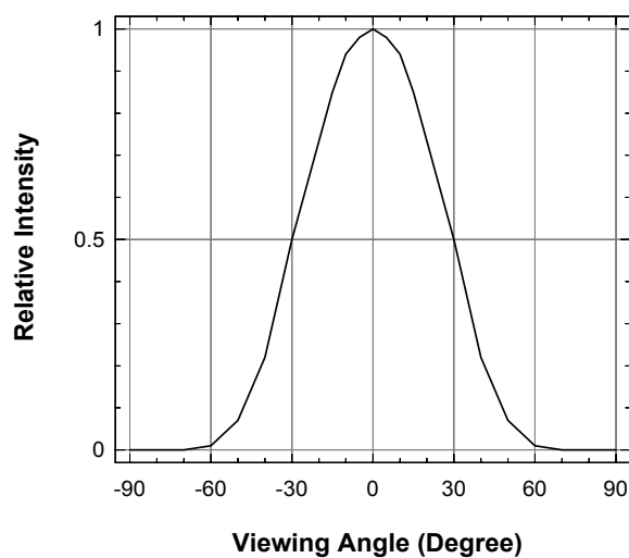
Radiation Pattern ( 2\theta=60^\circ )
