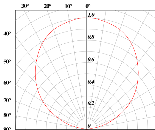
Radiation Pattern
