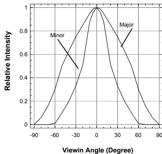
Radiation Pattern
