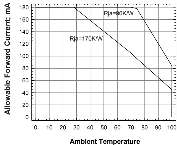
Foward Current Vs Ambient Temperature
