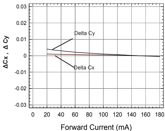
Chromaticity Vs Forward Current Test
