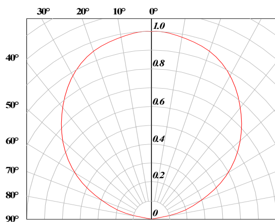
Radiation Pattern
