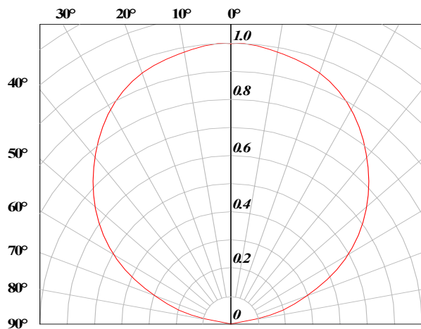
Radiation Pattern
