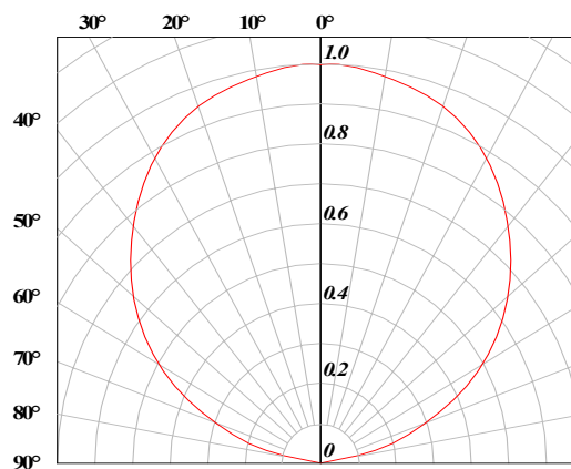
Radiation Pattern
