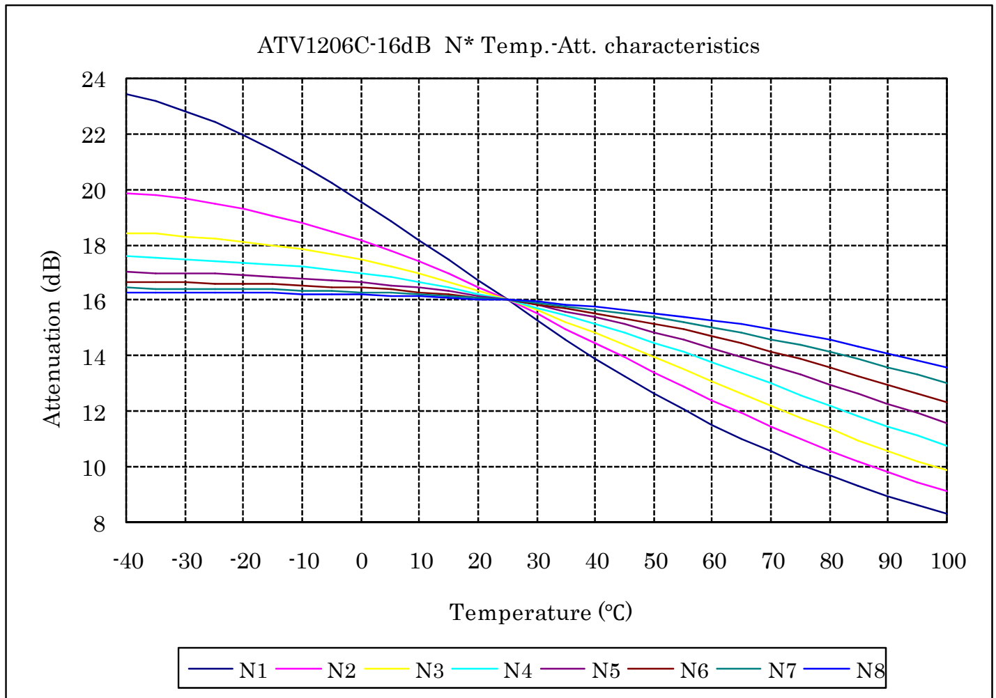
Attenuation at Temperatures Throughout Operating Temperature Range (16dB Product)
