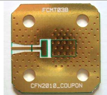
Material = Rogers 4250B, 10 mil thickness Call factory for DXF output of land pattern
