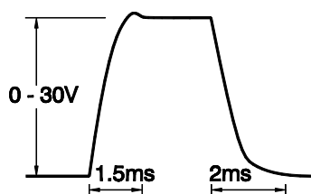
High programming speed of output voltage 30V in 1 ms (no electrolytic capacitors on output)
