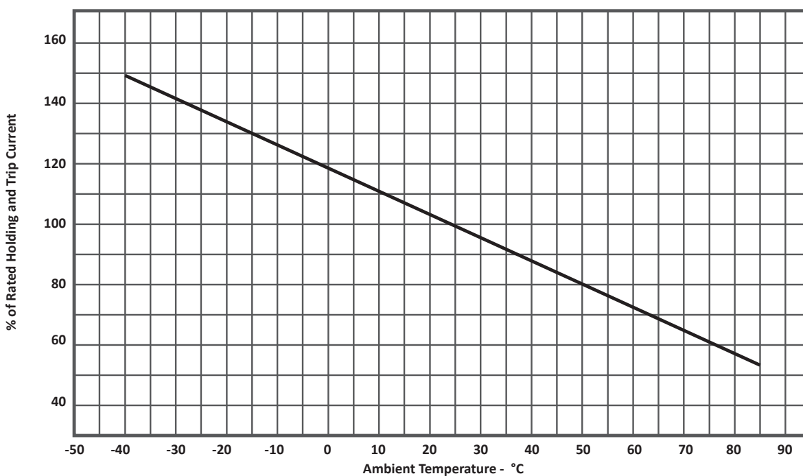
FIGURE 1 THERMAL DERATING CURVE (Rated Holding Current at Ambient Temperature)
