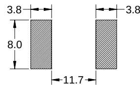
PCB PAD LAYOUT (REF.)
