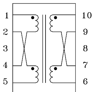
Circuit 1
