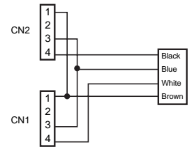
Wiring Diagram
