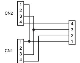
Wiring Diagram
