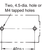
Mounting holes
