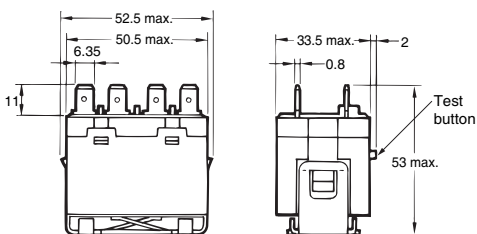
G7L-2A-TJ (with Test Button)
