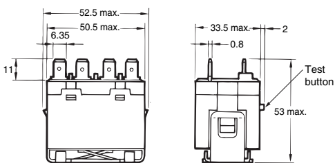
G7L-1A-TJ (with Test Button)
