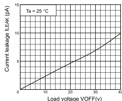
Current leakage vs. Load voltage I LEAK - VOFF
