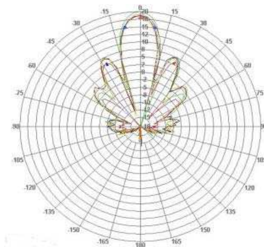
Antenna Pattern
