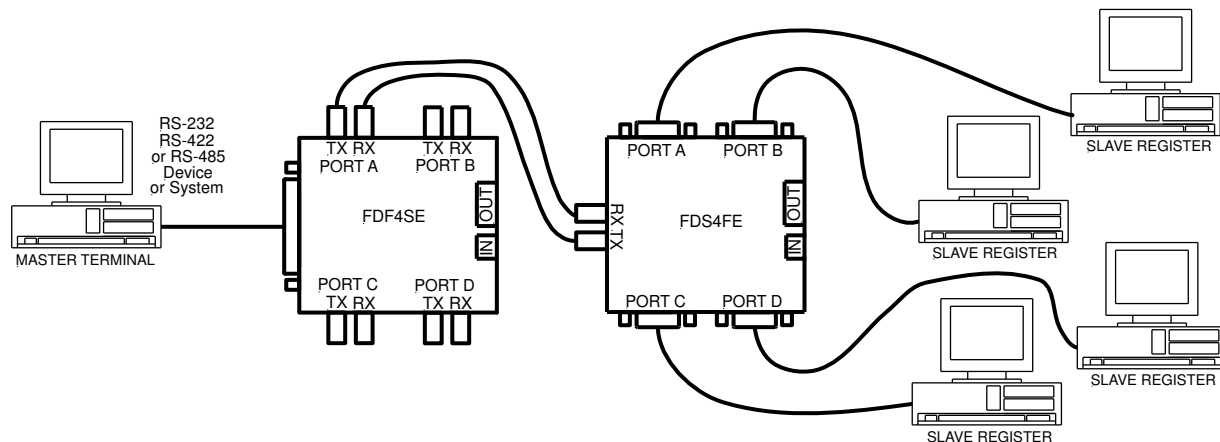
Figure 1: Typical Setup
