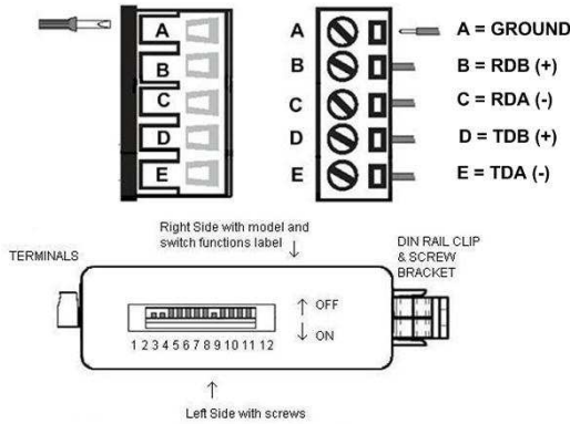
DIP Switch SW-1
