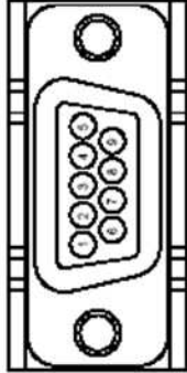
DB9 Male
