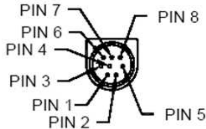
MINI-DIN 8 CONNECTOR
