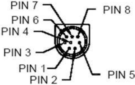
MINI-DIN 8 CONNECTOR
